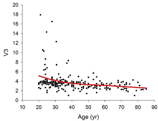
Supplemental Figure 1. Scatter plots showing the relationship between selected parameters of the base model and selected covariates. Parameter values are in black. Locally weighted scatterplot smoothing (LOWESS) lines are in red. Clearance = CL1; FFM = fat free mass which is calculated by the Janmahasatian et al formula. 24
