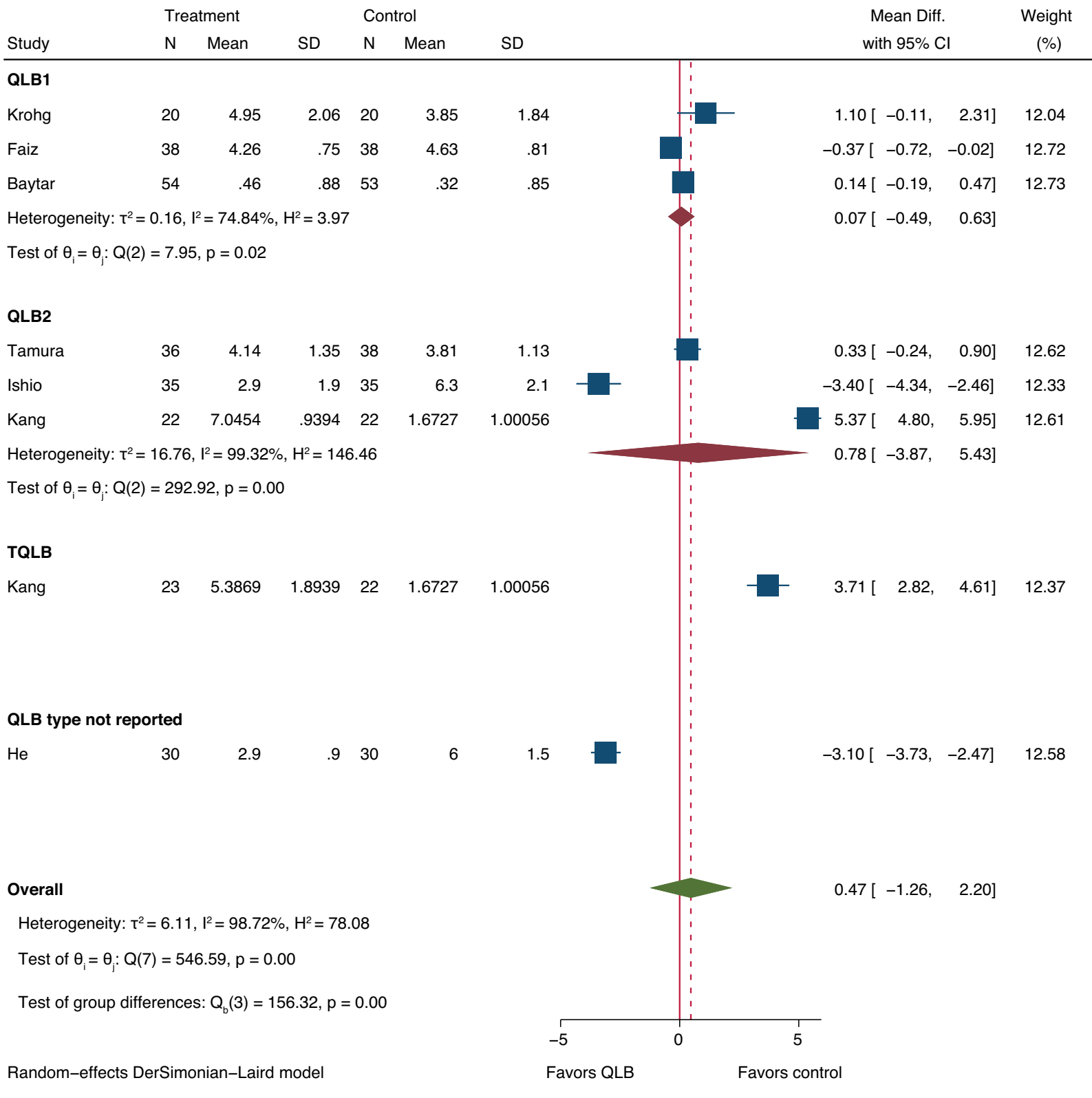
Figure S4. Forest plot showing the postoperative pain grade during movement at 24 hours. Subgroup analyses presented according to the QLB type. The sample size, mean, SDs and pooled estimates of mean difference (MD) are shown. The 95% CIs are shown as lines for individual studies and as diamonds for pooled estimates.
