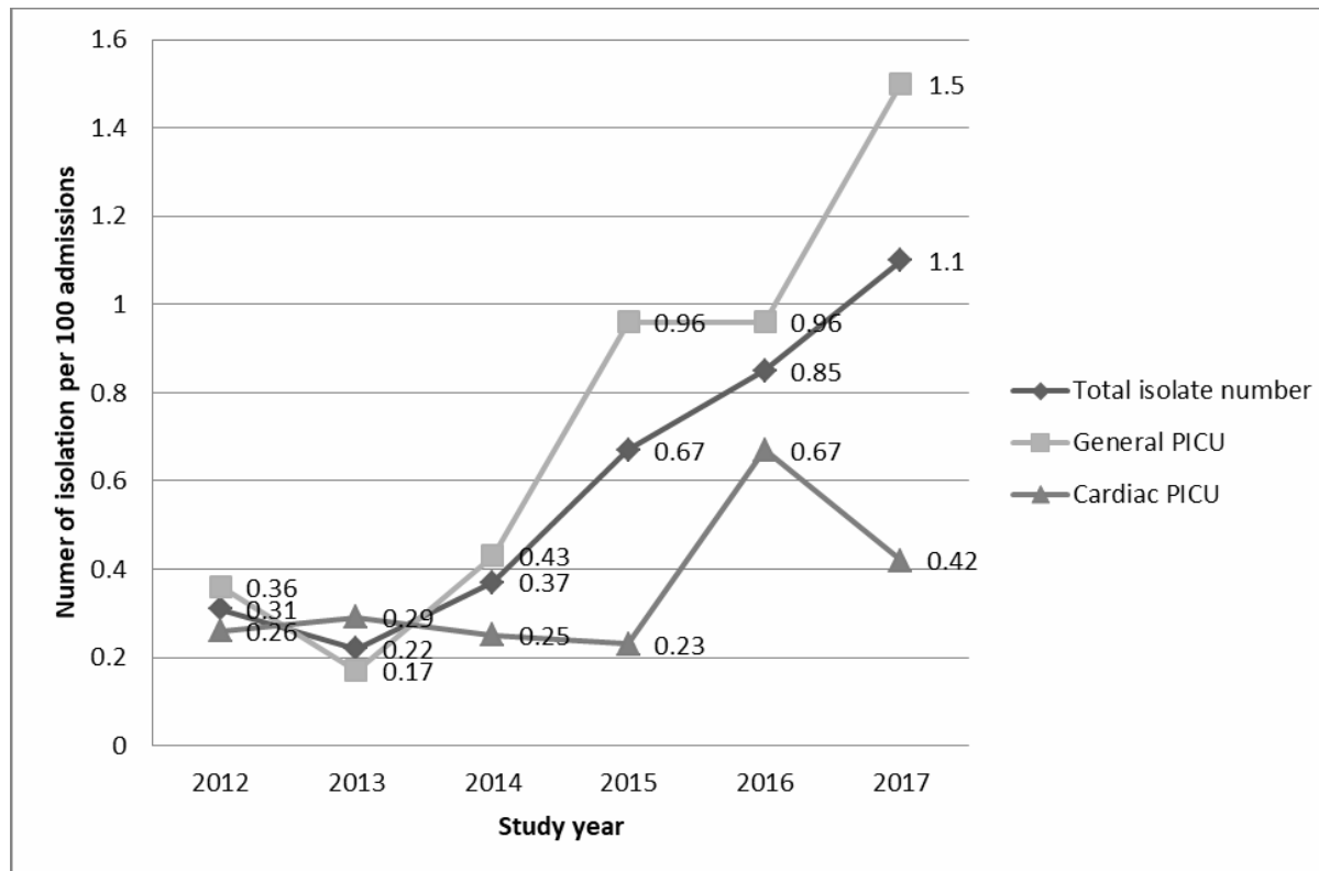
SDC 2. An illustration of the overall increase in incidence of the annual number of Stenotrophomonas maltophilia isolates per 100 admissions. The entire study group, the general pediatric intensive care unit and the cardiac pediatric intensive care unit are presented separately. PICU: pediatric intensive care unit.
