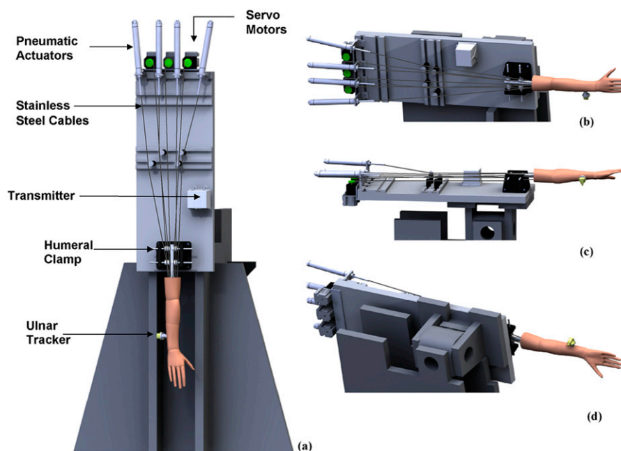
Fig. E-1 Schematic representations of the elbow motion simulator, containing a mounted specimen (a pronated right arm), in vertical ( Fig. E-1A ), valgus ( Fig. E-1B ), horizontal ( Fig. E-1C ), and varus ( Fig. E-1D ) orientations.
