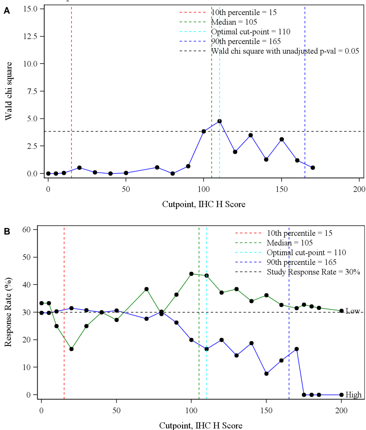
Supplementary Figure 7: Wald chi-square statistic (A) and ORR (B) plotted versus each cytoplasm TS H-score as cut-point chosen to divide patients into low and high expression groups (N = 60)
