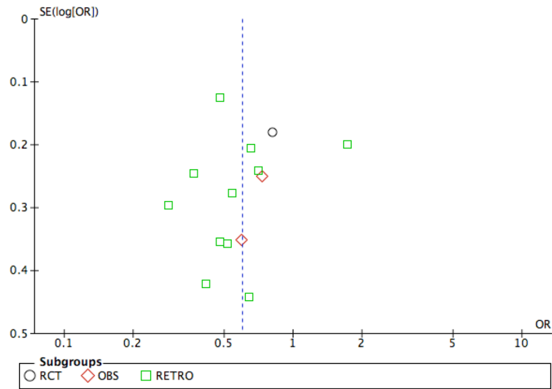
SDC Figure 5: Funnel plot for High vs. Low PLAS:RBC Ratio.
