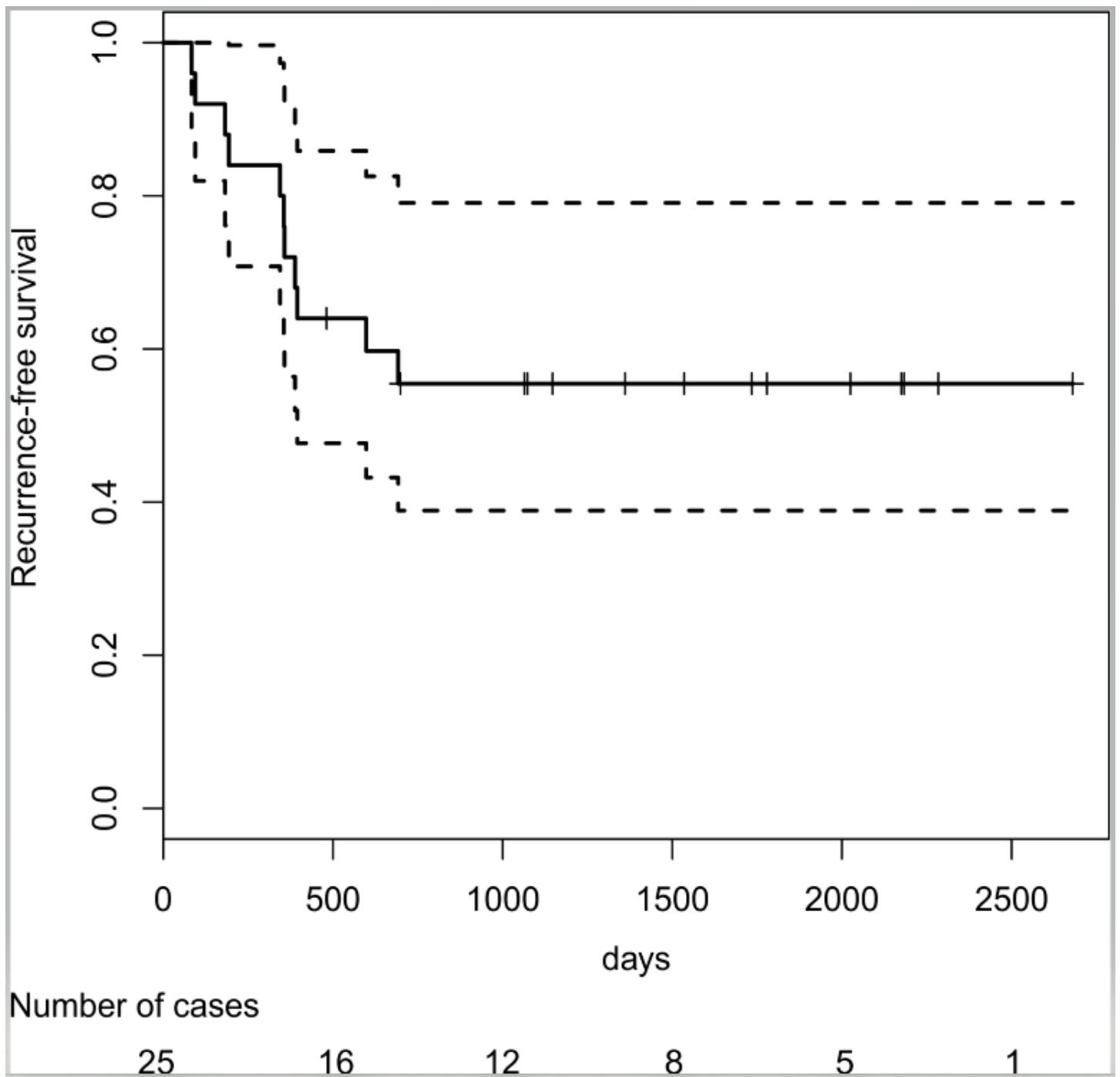
Figure S1: Kaplan-Meier curve of recurrence-free survival in the of the study cohort (solid line) with the corresponding 95% confidence interval (dotted lines).
