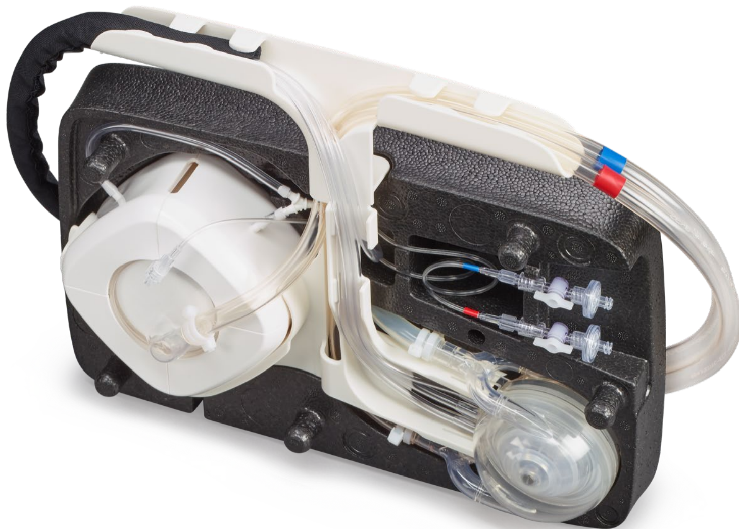
Supplemental Image 3: View inside the MobyBox: Technical inner life of the Patient unit with the oxygenator on the left side and the displacement pump in the lower right corner.
