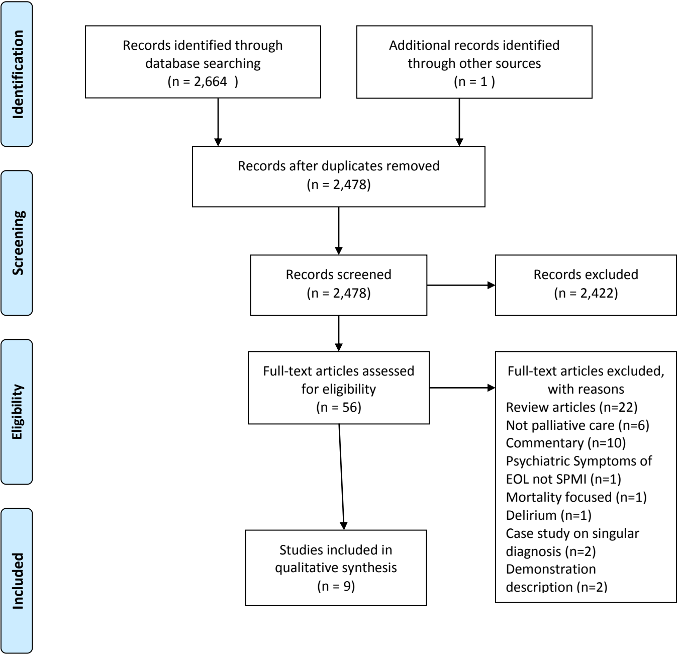
Figure 1. PRISMA Diagram.
