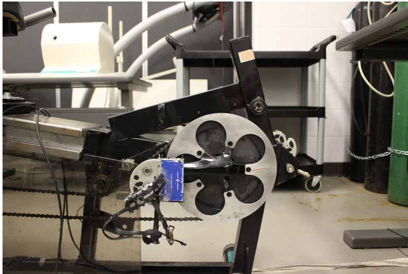
Supplementary Digital Content 1. Pictures of the new cycling ergometer. (A) View of cycling ergometer from behind. (B) View of cycling ergometer from the side. (C) View of force pedal. (D) View of locked force pedal and foot with the ankle in the contraction position.
