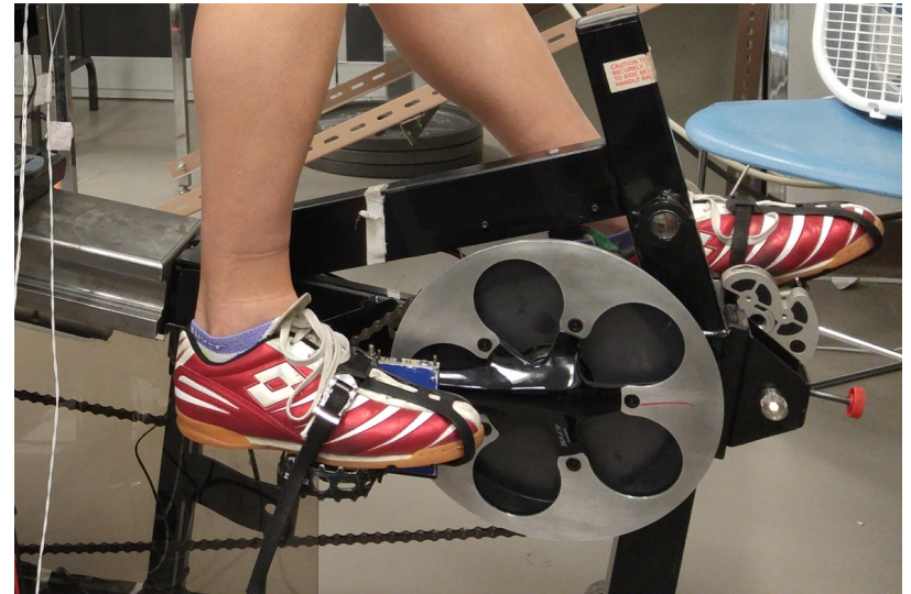
Supplementary Digital Content 1. Pictures of the new cycling ergometer. (A) View of cycling ergometer from behind. (B) View of cycling ergometer from the side. (C) View of force pedal. (D) View of locked force pedal and foot with the ankle in the contraction position.
