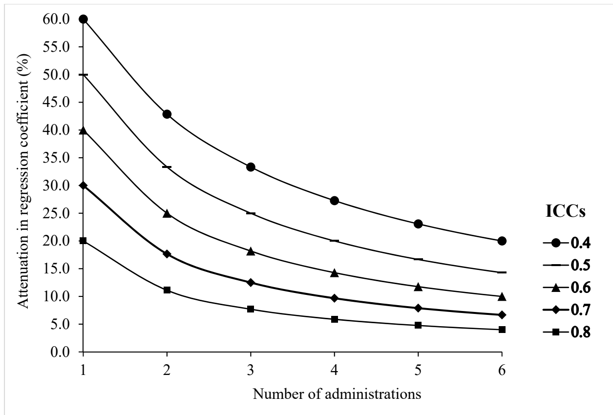
Figure S2. The percentage attenuation (y-axis) in the expected estimate of the regression coefficient as the number of administrations (x-axis) increases for ICCs ranging from 0.4 to 0.8.
