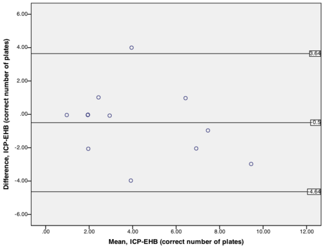
Figure E3. Bland-Altman plot depicting agreement of values for correct number of plates measured by the Eye Handbook (EHB) Color Vision Test and Ishihara Color Plates (ICP) in color vision deficient subjects. The upper and lower lines are at the 95 th percentile of differences in score.
